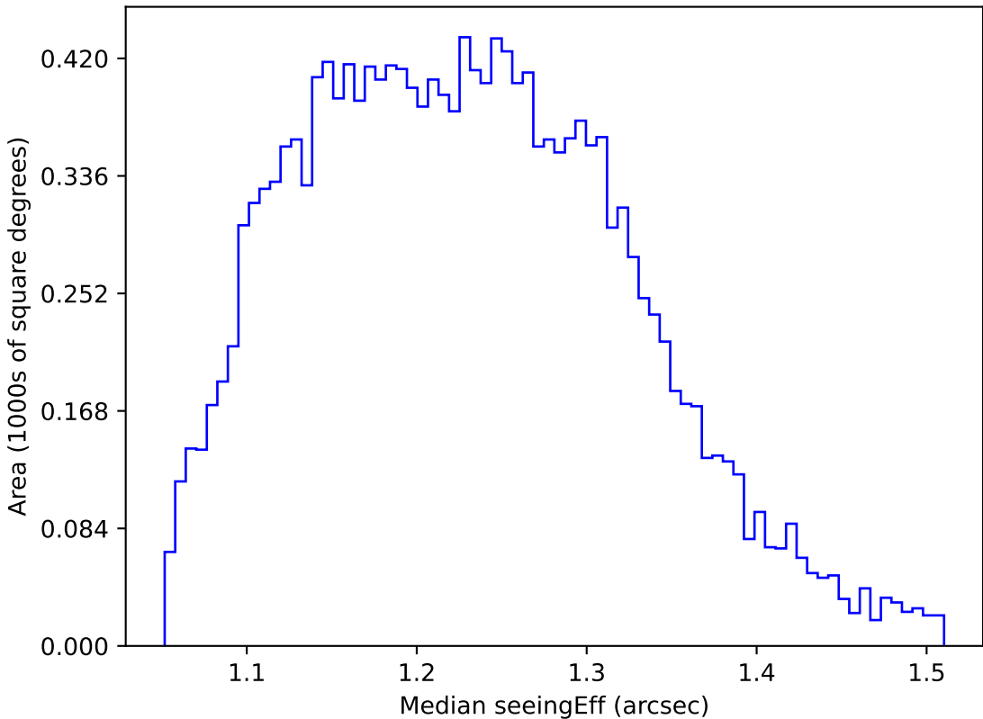
too_ignore_100_4v3.4_10yrs WFD u band: Median seeingEff
