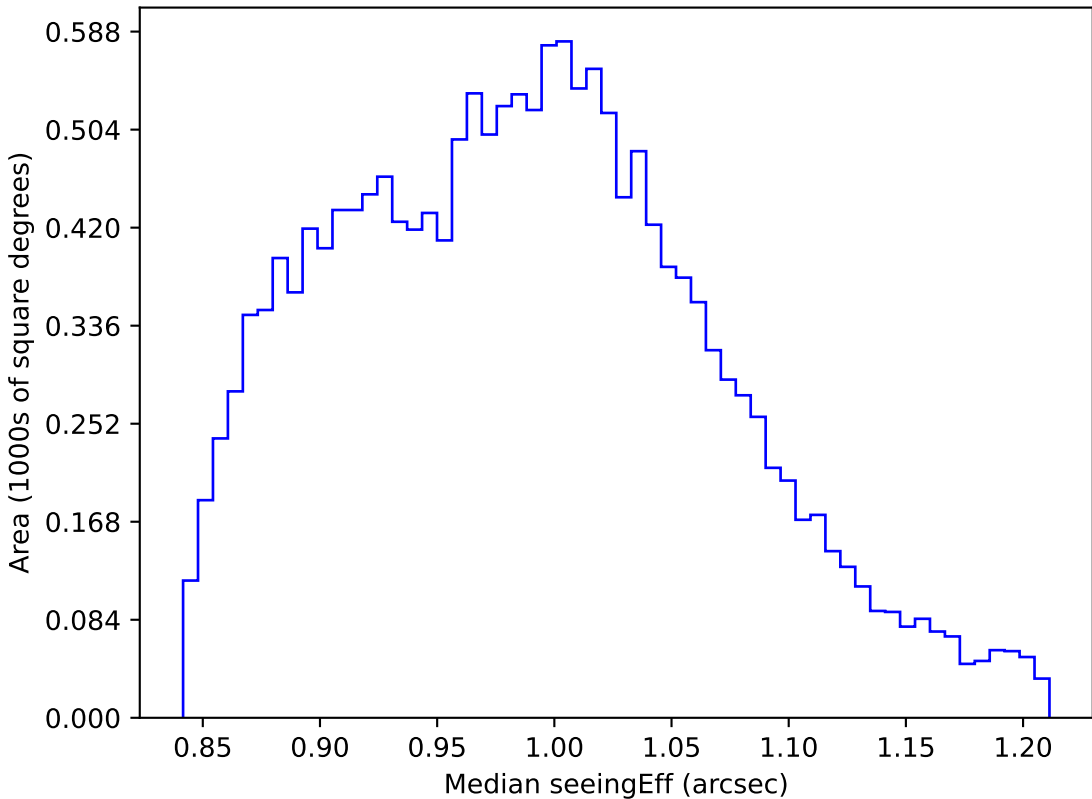
too_ignore_100_4v3.4_10yrs WFD i band: Median seeingEff
