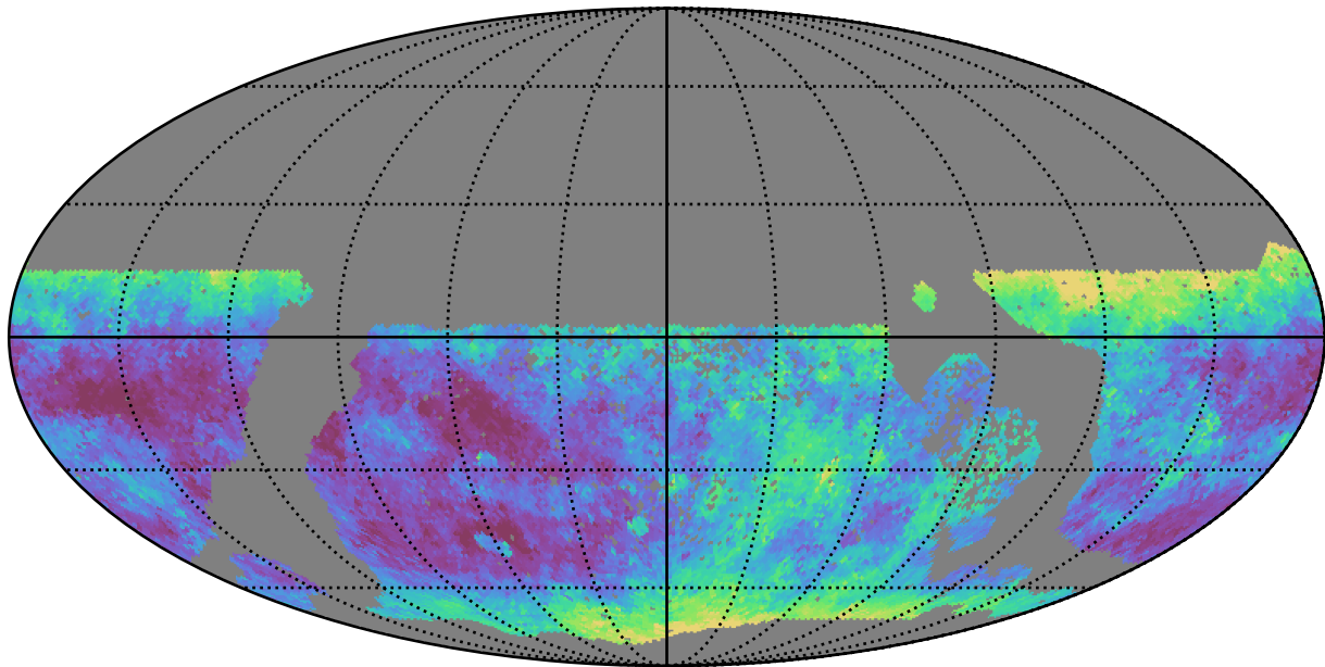
too_ignore_100_4v3.4_10yrs WFD g band: Median seeingEff
