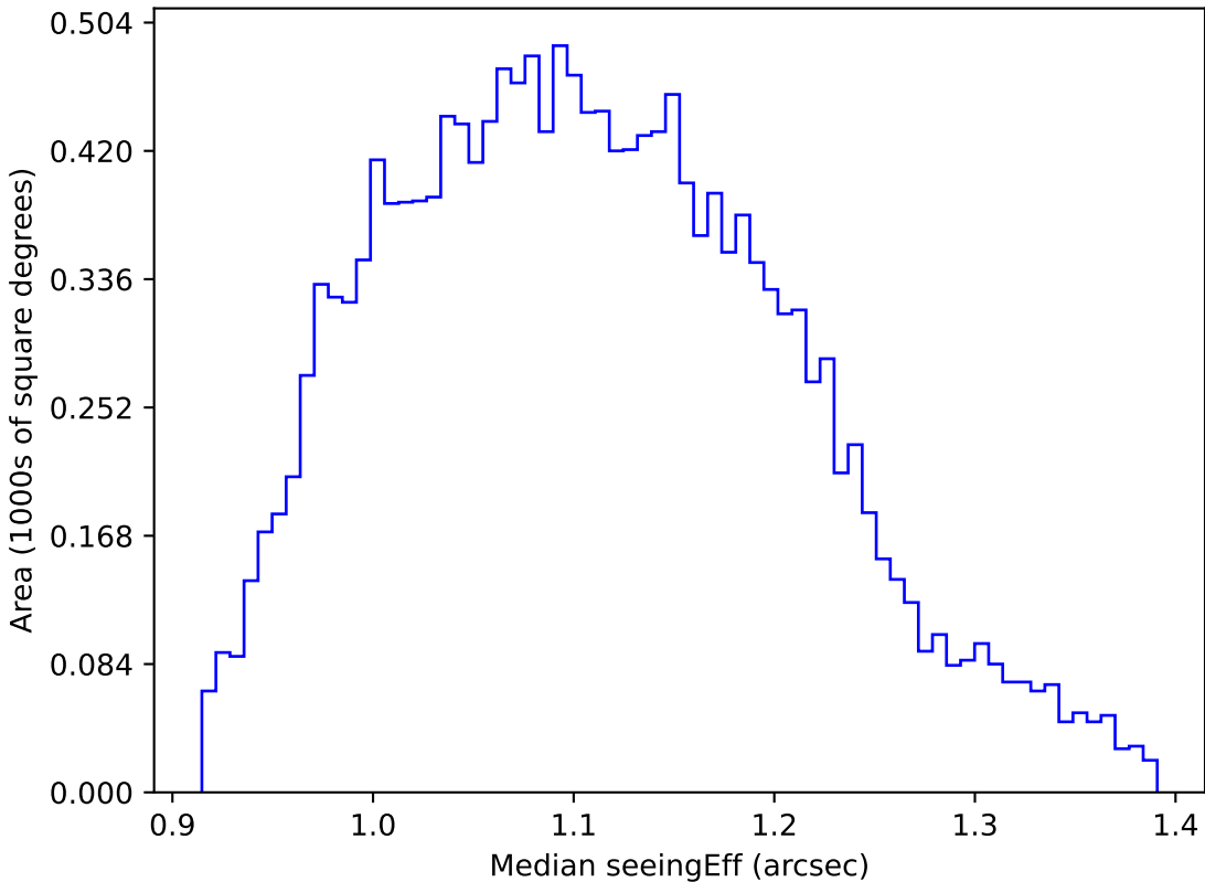
too_ignore_100_4v3.4_10yrs WFD g band: Median seeingEff
