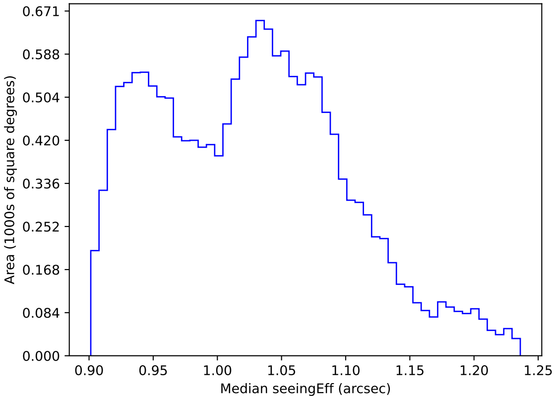
too_ignore_100_4v3.4_10yrs WFD all bands: Median seeingEff
