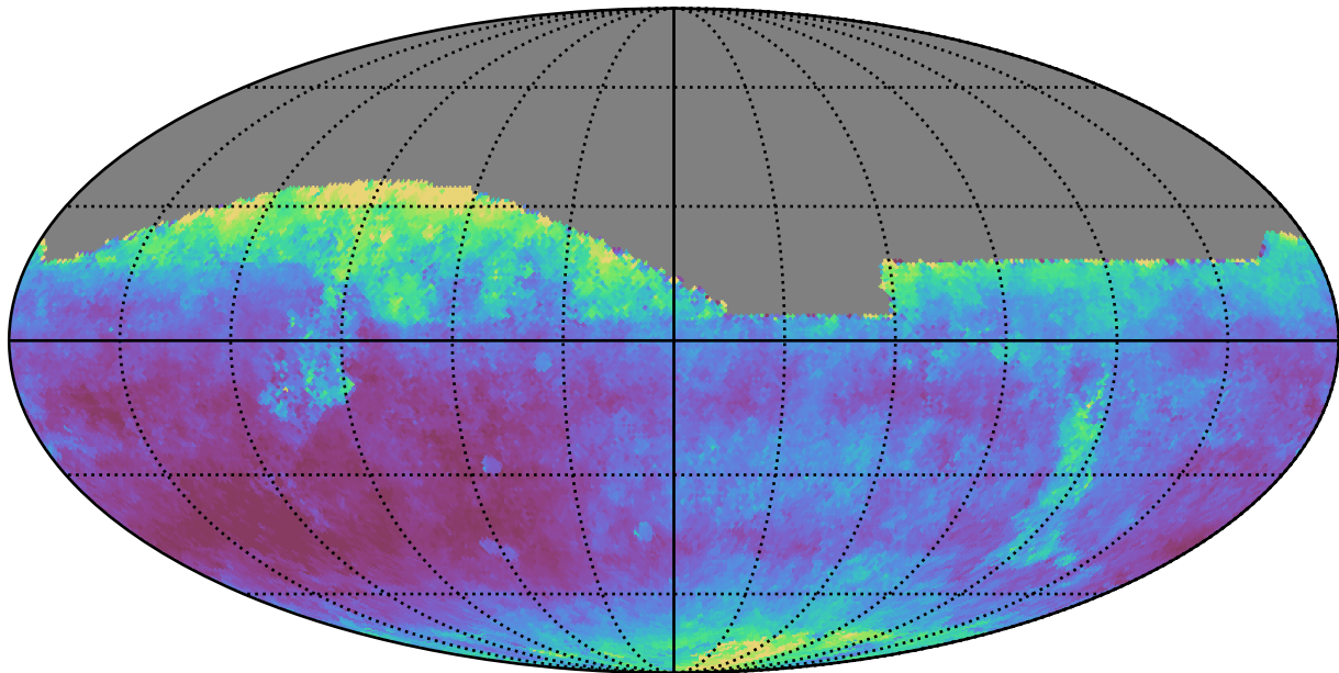
too_ignore_100_4v3.4_10yrs All sky z band: Median seeingEff
