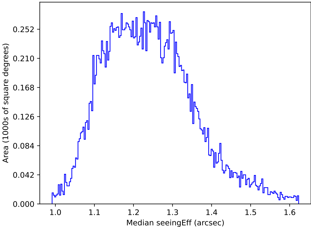
too_ignore_100_4v3.4_10yrs All sky u band: Median seeingEff
