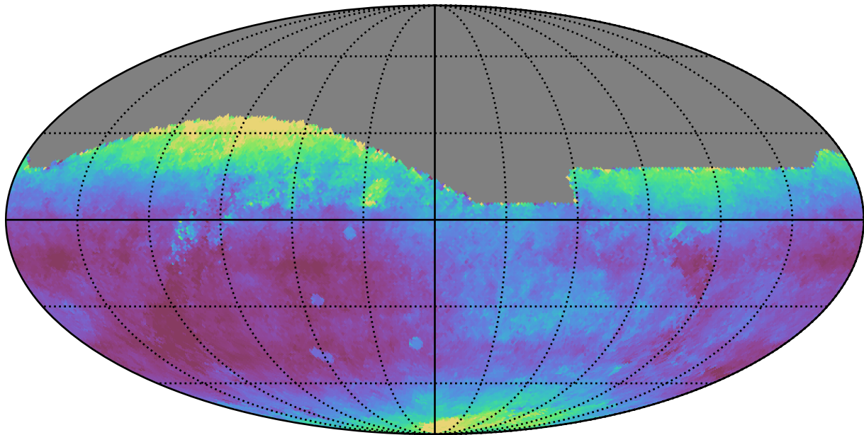
too_ignore_100_4v3.4_10yrs All sky r band: Median seeingEff
