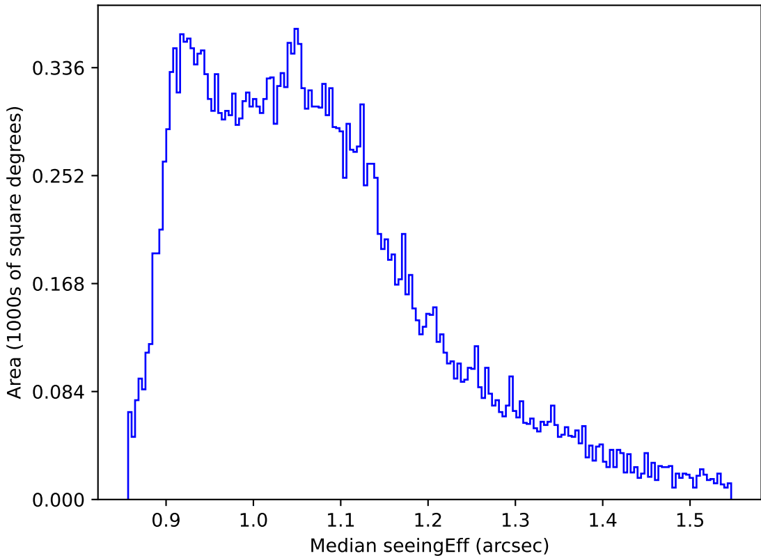
too_ignore_100_4v3.4_10yrs All sky r band: Median seeingEff
