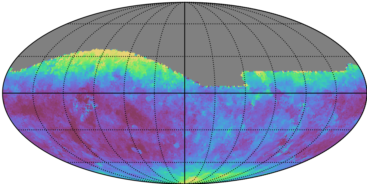
too_ignore_100_4v3.4_10yrs All sky g band: Median seeingEff
