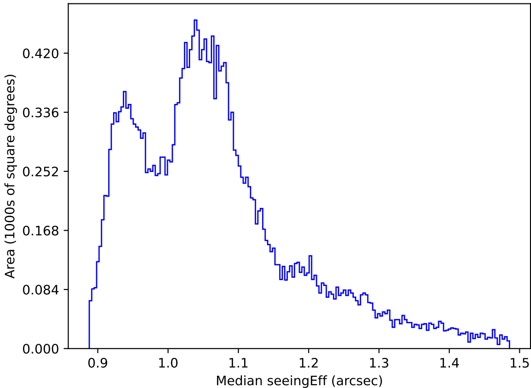
too_ignore_100_4v3.4_10yrs All sky all bands: Median seeingEff
