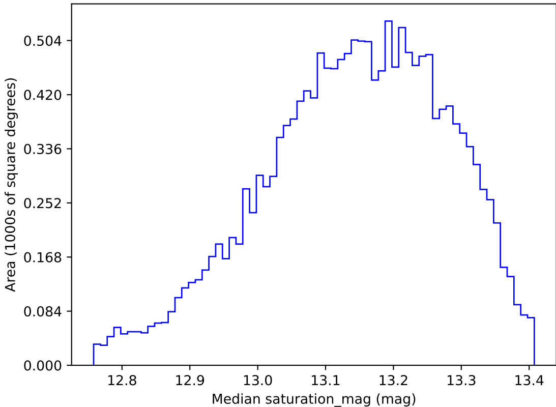
too_ignore_100_4v3.4_10yrs WFD y band: Median saturation_mag
