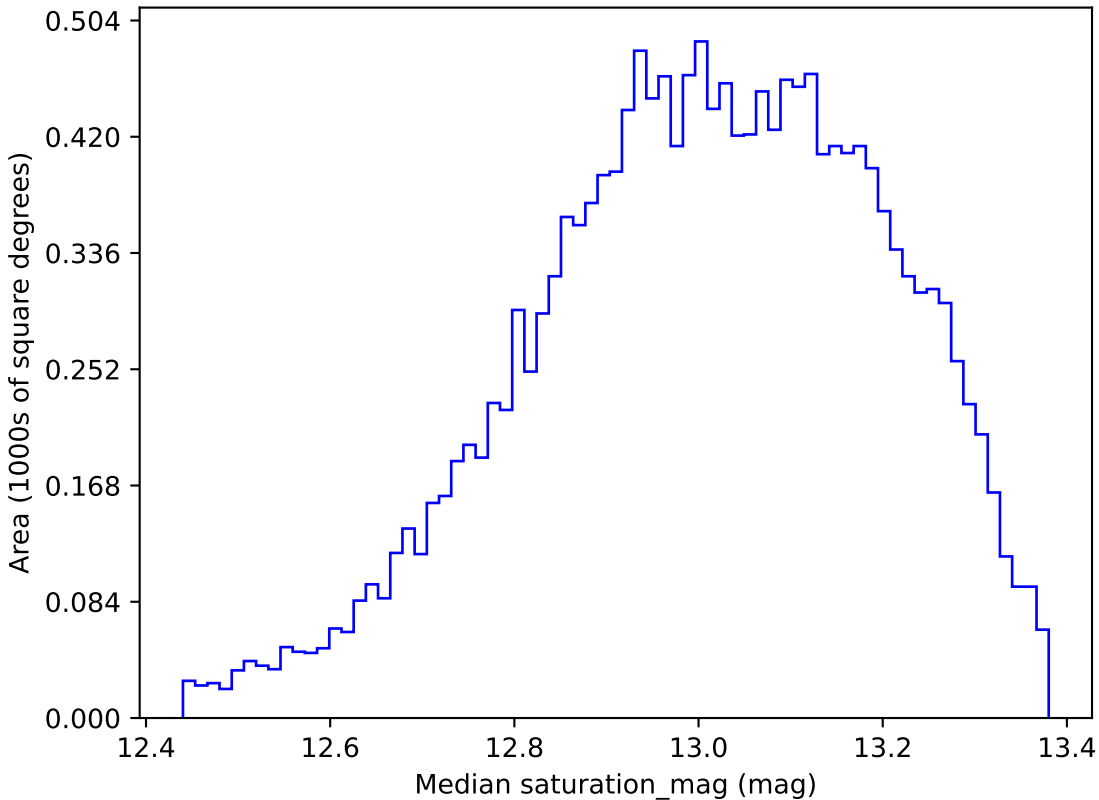
too_ignore_100_4v3.4_10yrs WFD u band: Median saturation_mag
