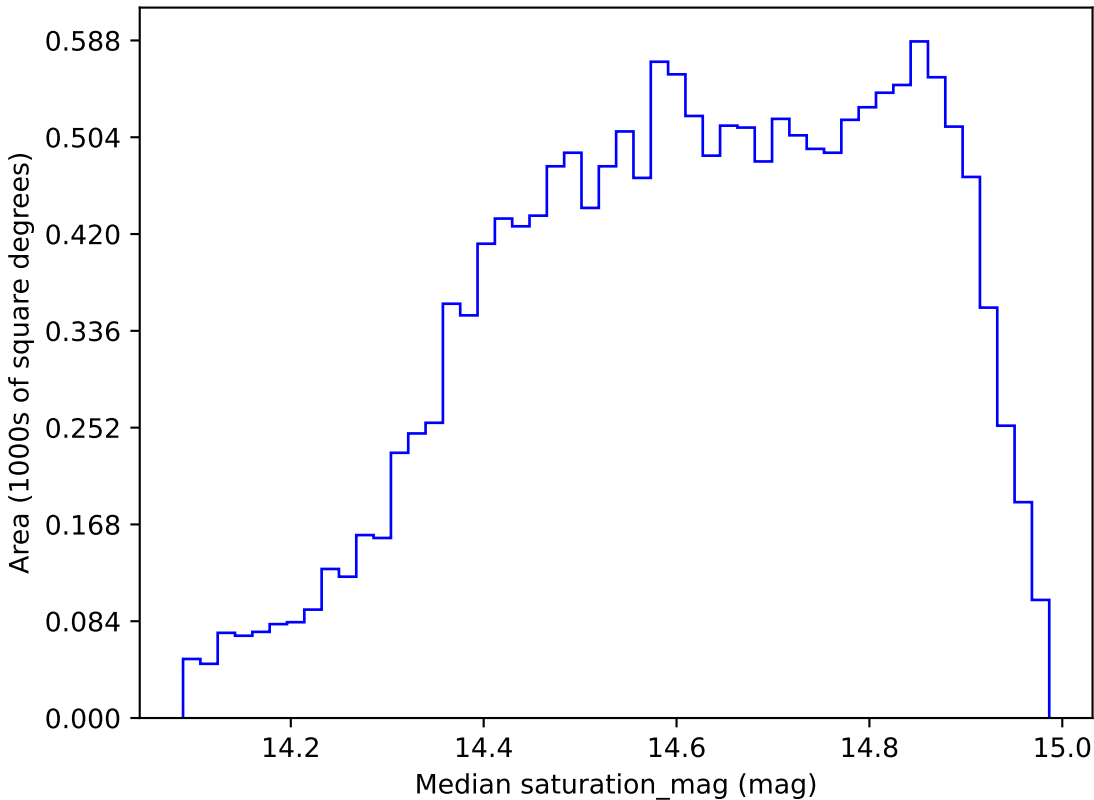
too_ignore_100_4v3.4_10yrs WFD r band: Median saturation_mag
