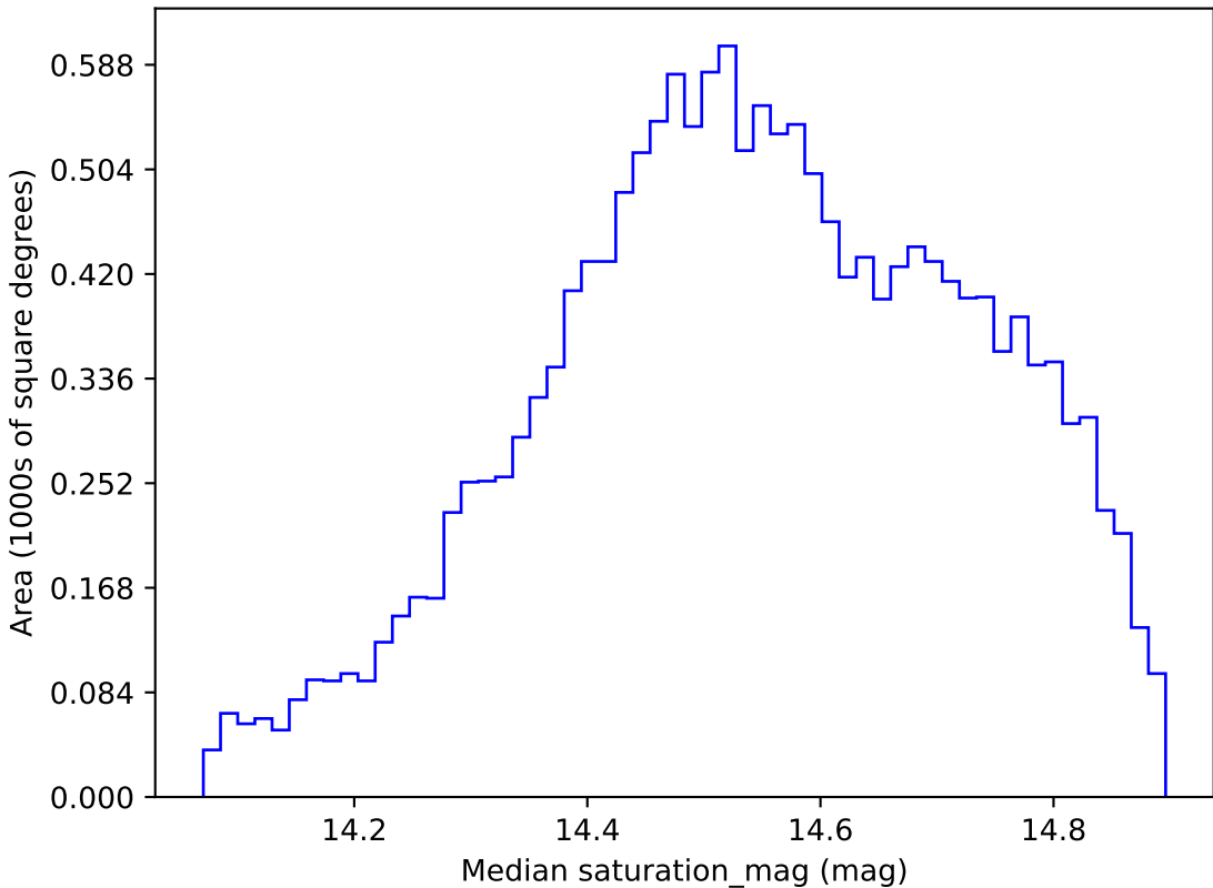
too_ignore_100_4v3.4_10yrs WFD i band: Median saturation_mag
