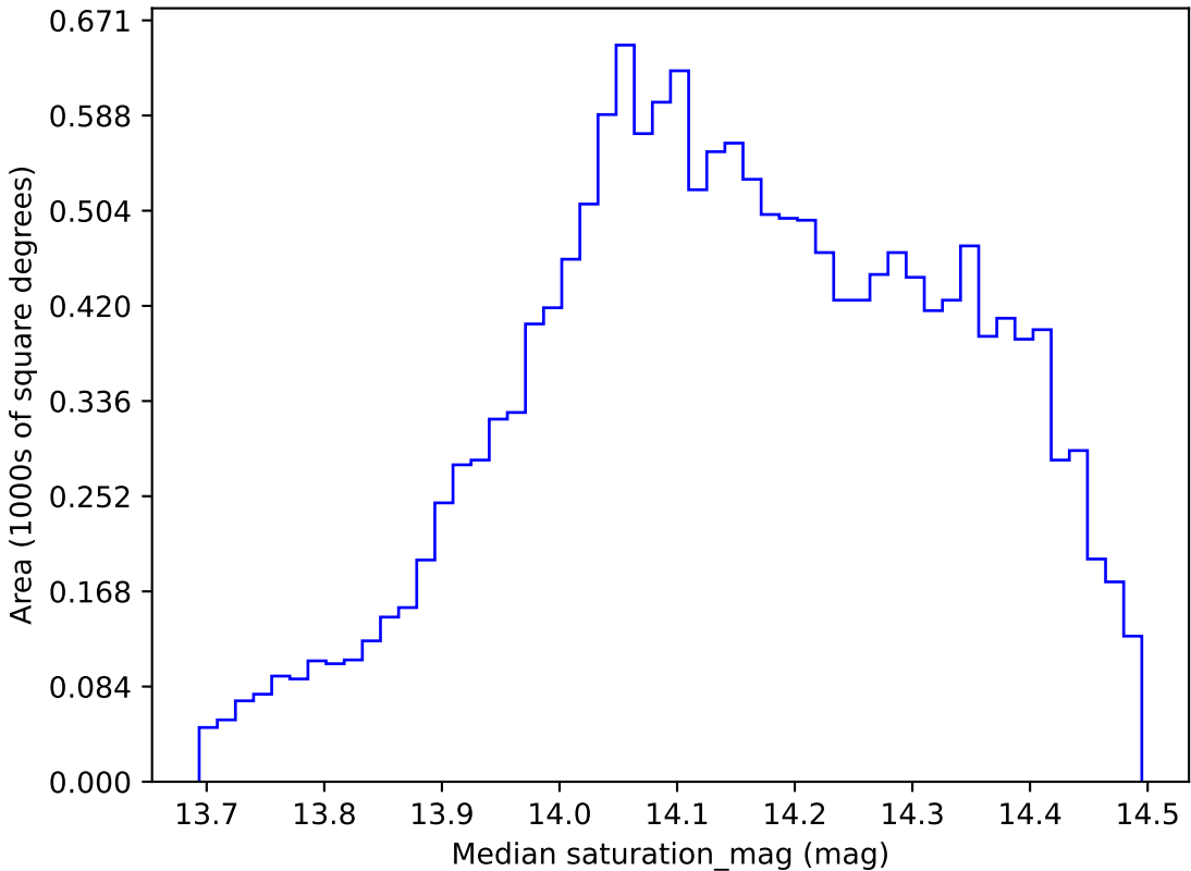
too_ignore_100_4v3.4_10yrs WFD all bands: Median saturation_mag
