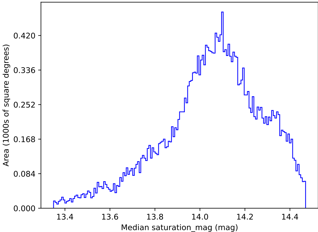
too_ignore_100_4v3.4_10yrs All sky z band: Median saturation_mag
