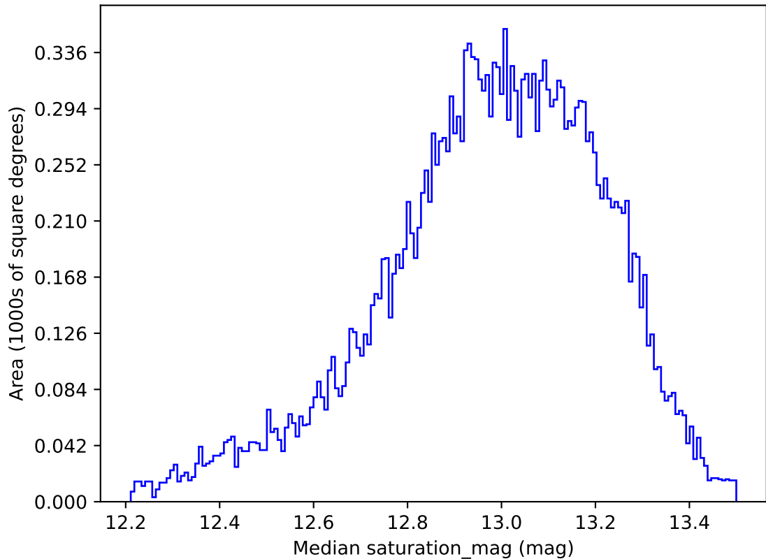
too_ignore_100_4v3.4_10yrs All sky u band: Median saturation_mag
