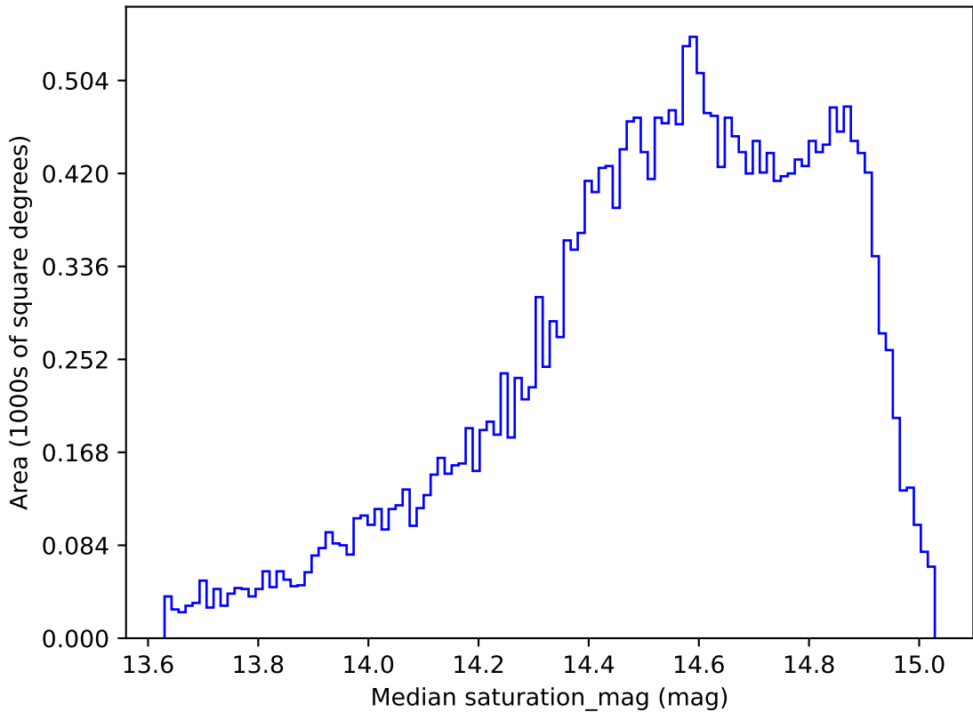
too_ignore_100_4v3.4_10yrs All sky r band: Median saturation_mag
