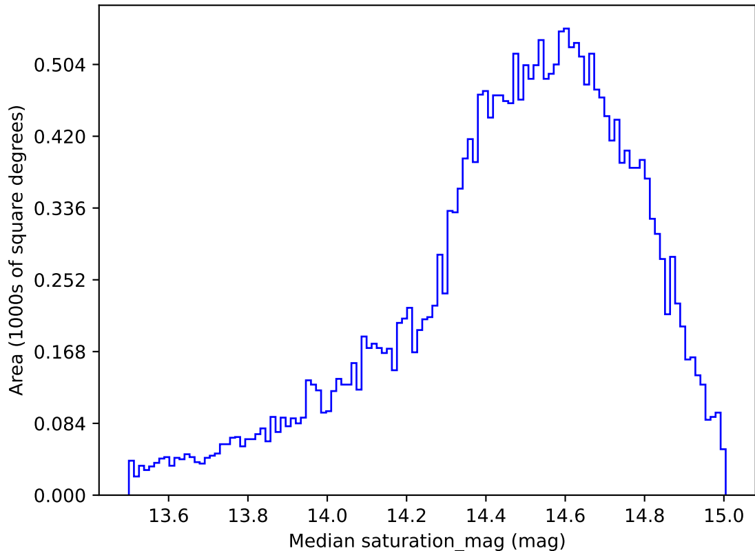
too_ignore_100_4v3.4_10yrs All sky g band: Median saturation_mag
