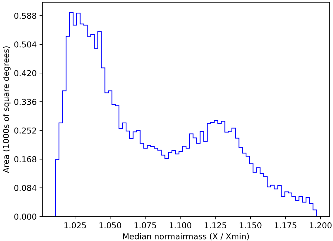
too_ignore_100_4v3.4_10yrs WFD u band: Median normairmass
