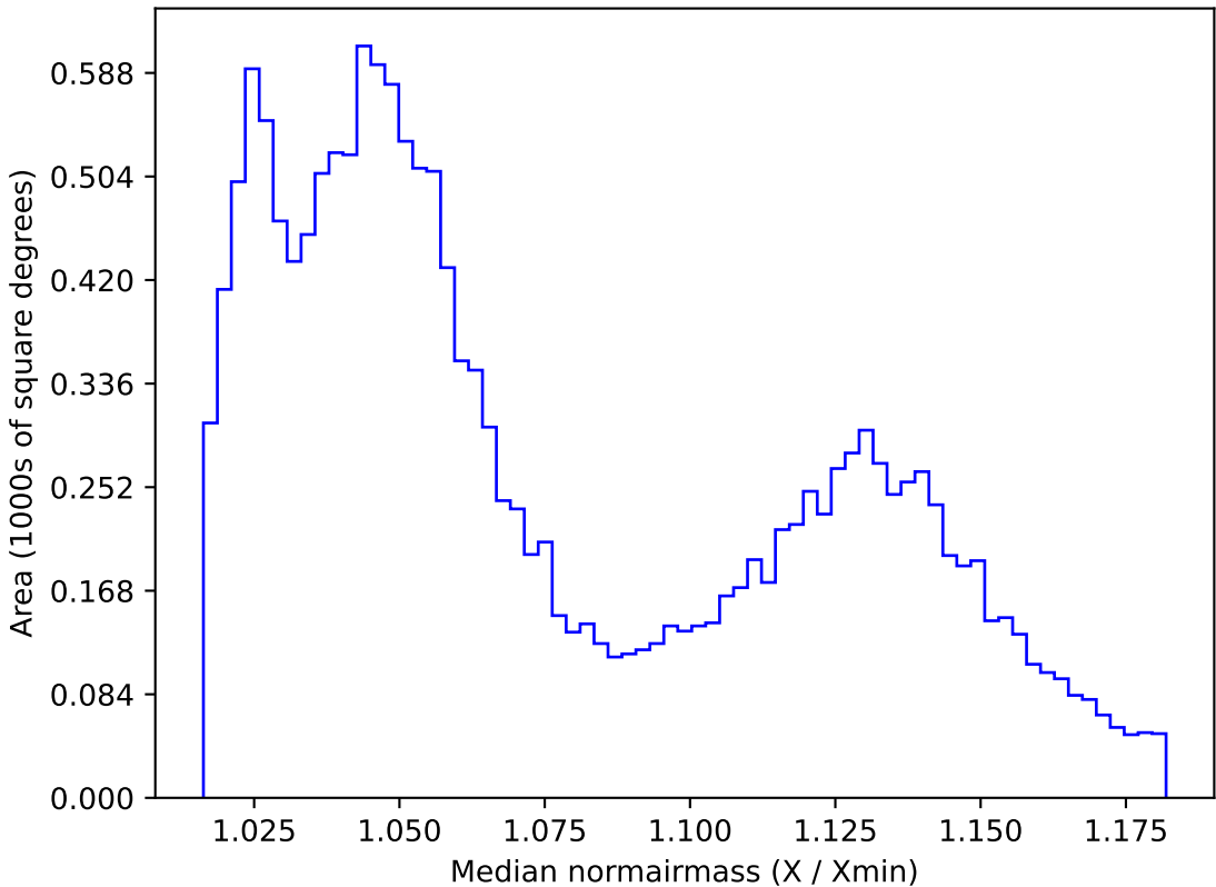
too_ignore_100_4v3.4_10yrs WFD r band: Median normairmass
