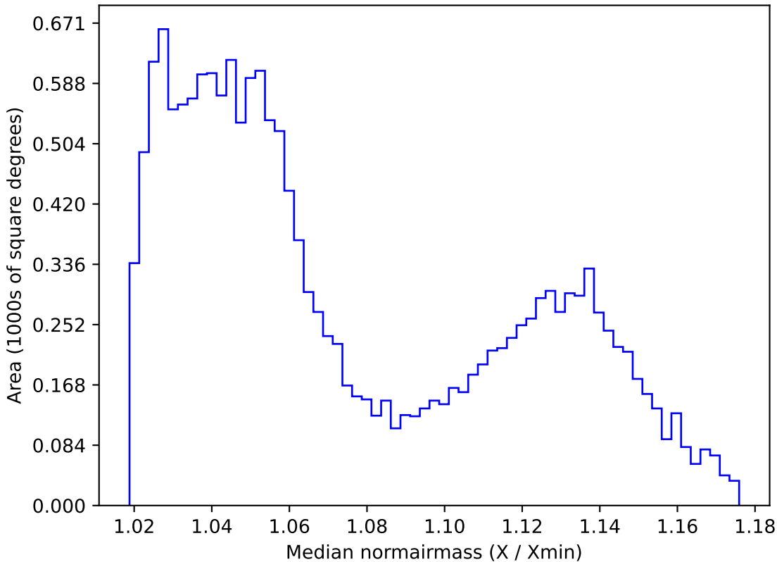
too_ignore_100_4v3.4_10yrs WFD i band: Median normairmass
