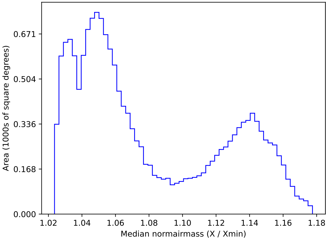
too_ignore_100_4v3.4_10yrs WFD all bands: Median normairmass
