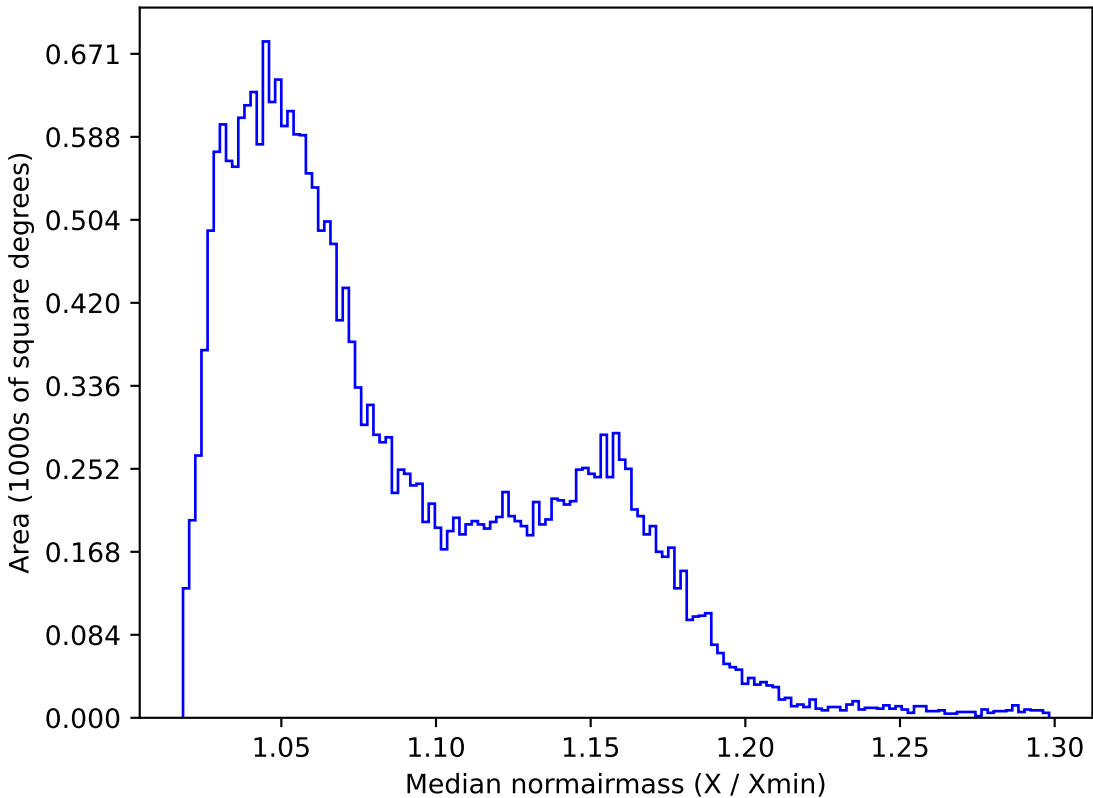
too_ignore_100_4v3.4_10yrs All sky z band: Median normairmass
