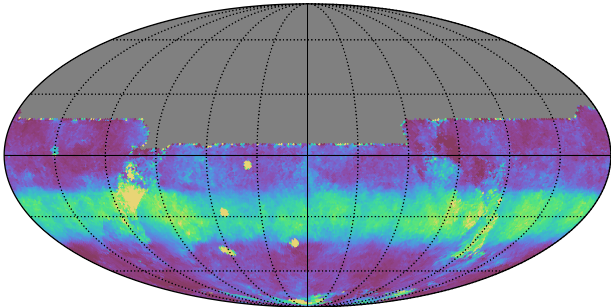
too_ignore_100_4v3.4_10yrs All sky y band: Median normairmass
