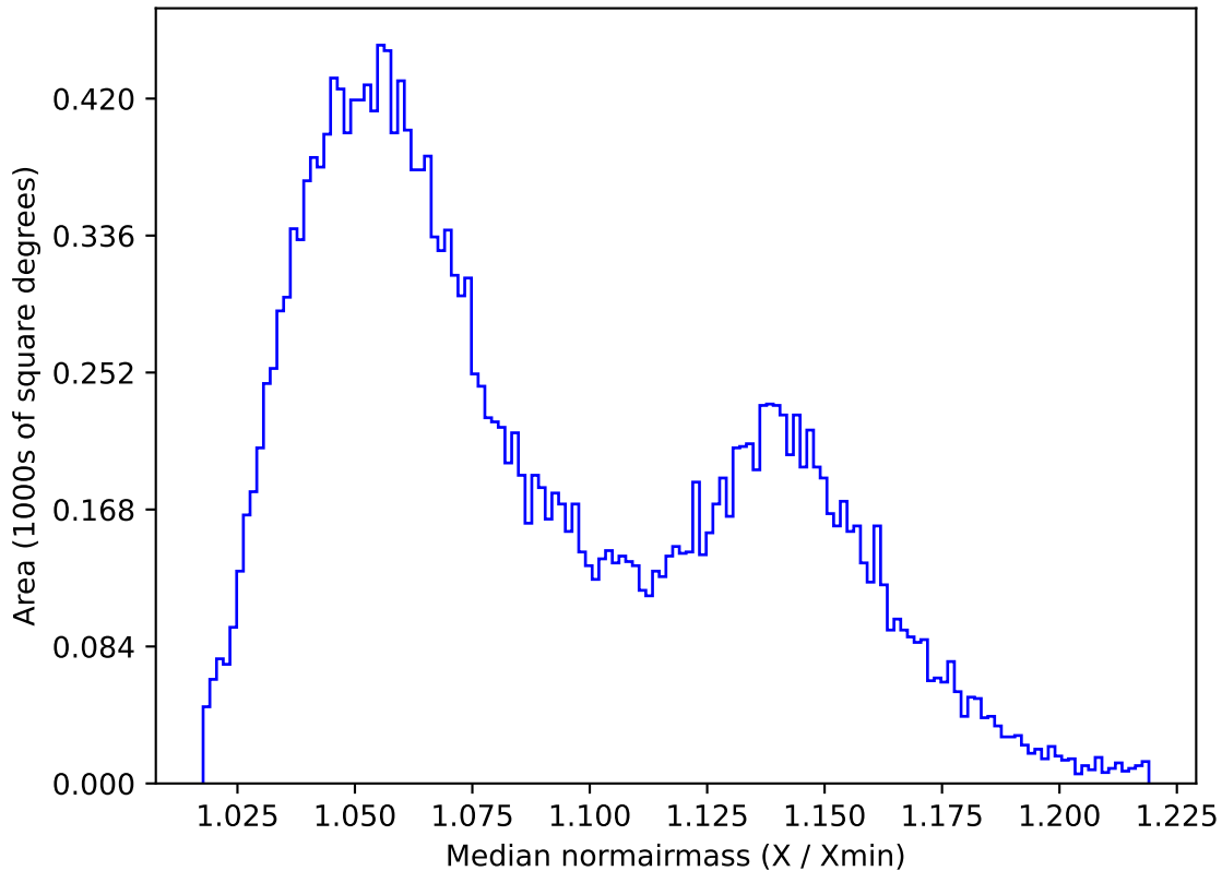
too_ignore_100_4v3.4_10yrs All sky y band: Median normairmass
