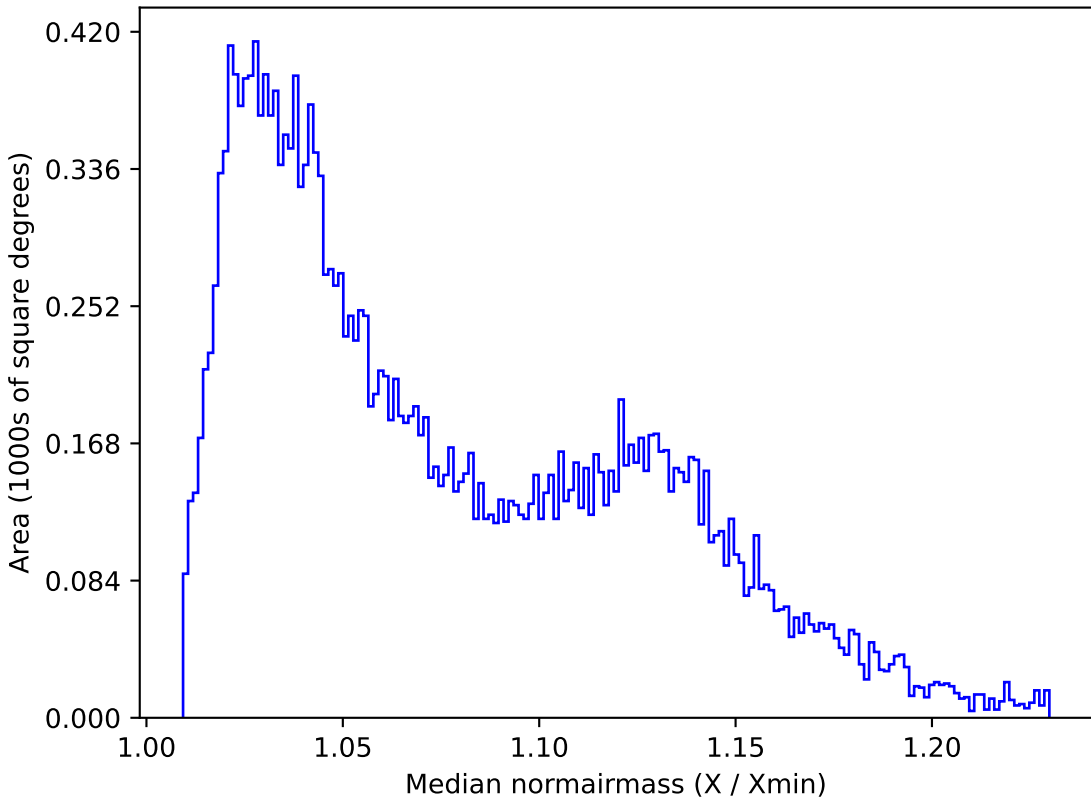
too_ignore_100_4v3.4_10yrs All sky u band: Median normairmass
