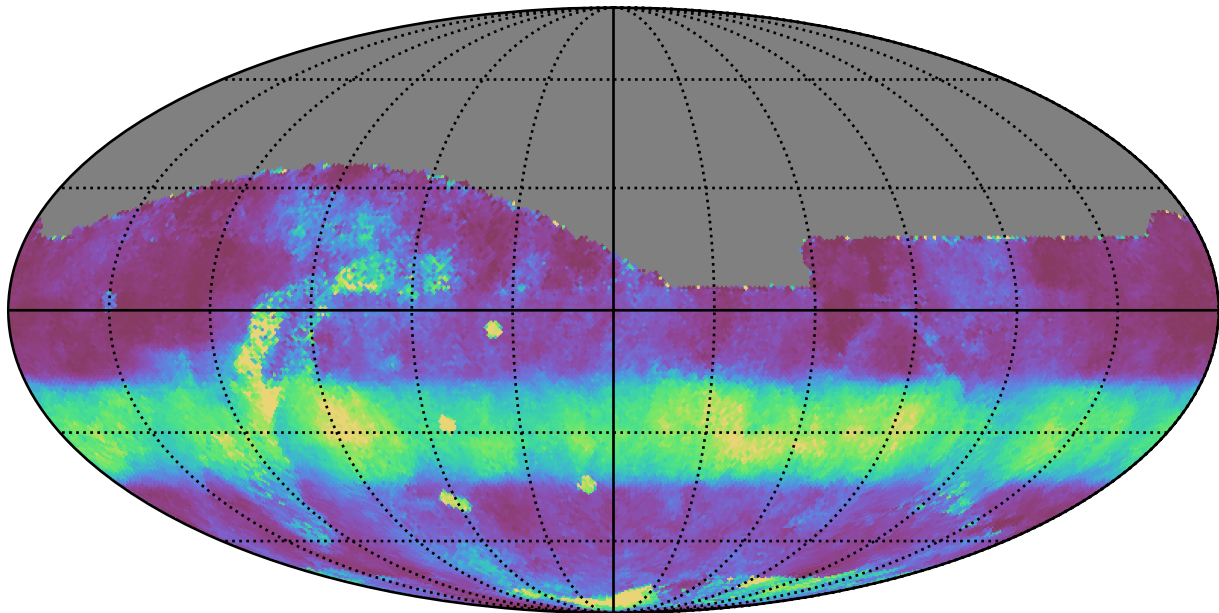
too_ignore_100_4v3.4_10yrs All sky r band: Median normairmass
