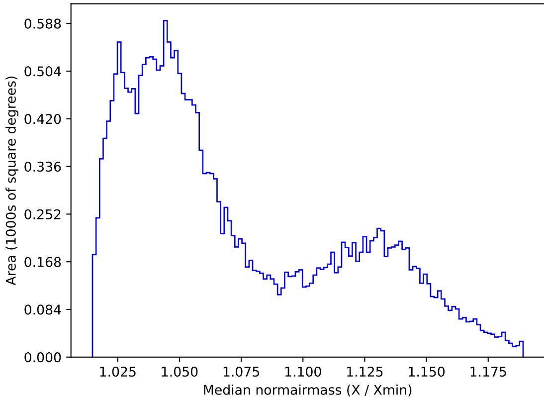
too_ignore_100_4v3.4_10yrs All sky r band: Median normairmass
