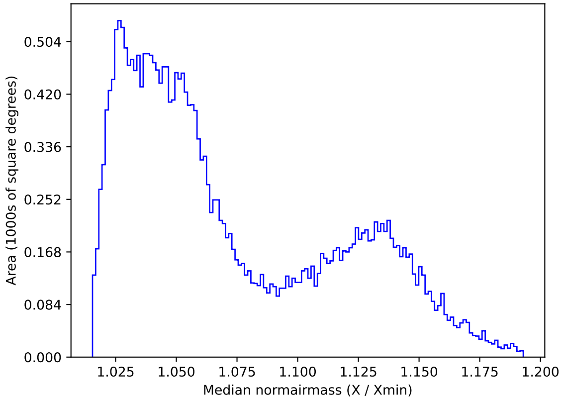
too_ignore_100_4v3.4_10yrs All sky i band: Median normairmass
