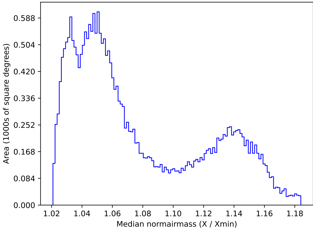
too_ignore_100_4v3.4_10yrs All sky all bands: Median normairmass
