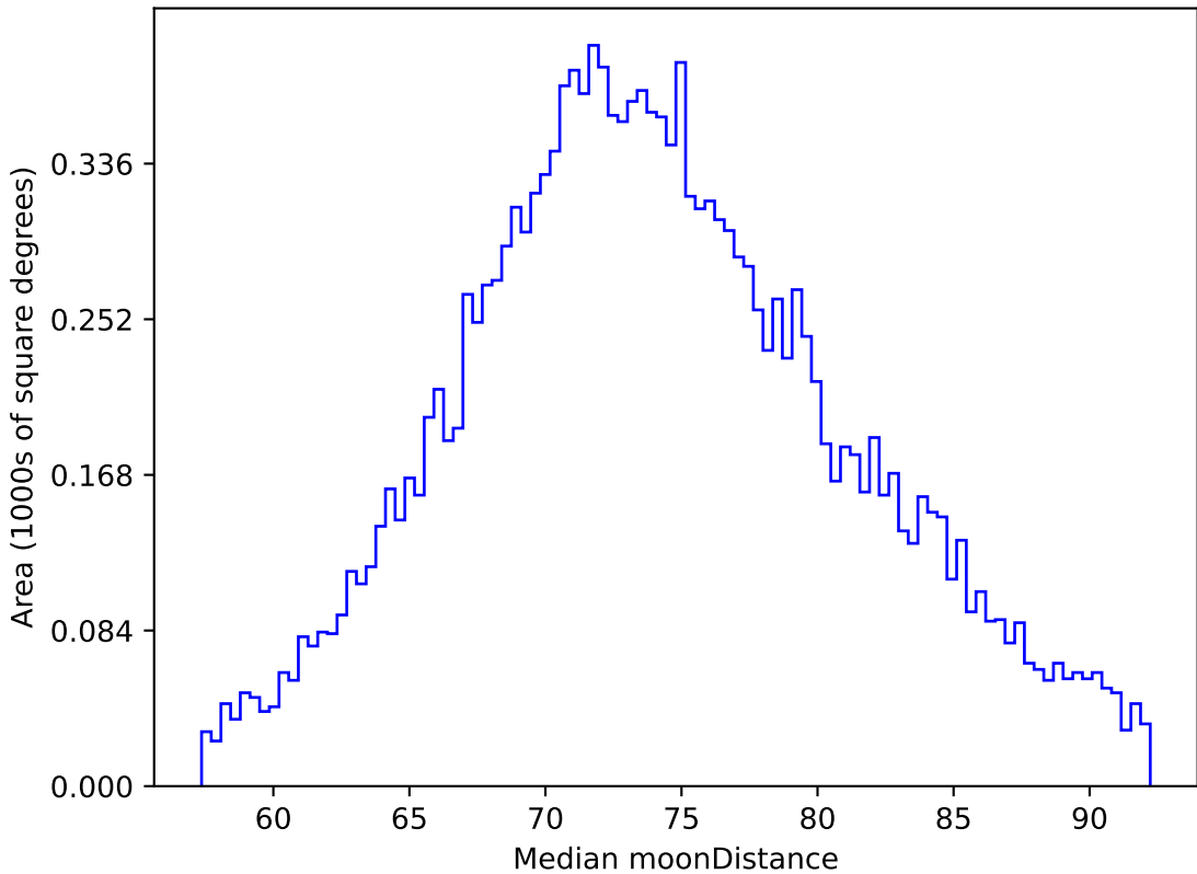
too_ignore_100_4v3.4_10yrs WFD z band: Median moonDistance
