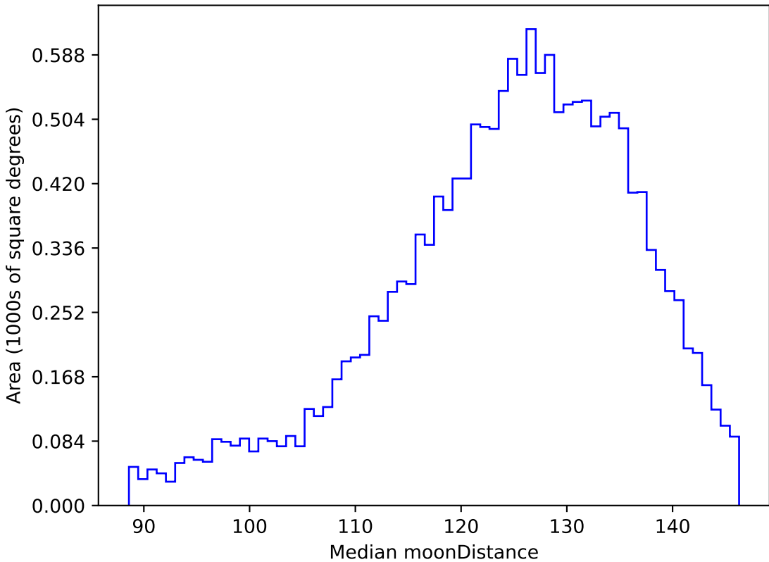
too_ignore_100_4v3.4_10yrs WFD u band: Median moonDistance
