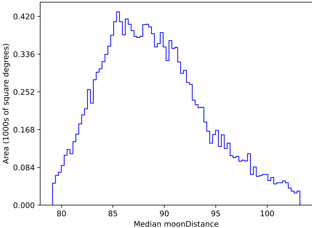
too_ignore_100_4v3.4_10yrs WFD all bands: Median moonDistance
