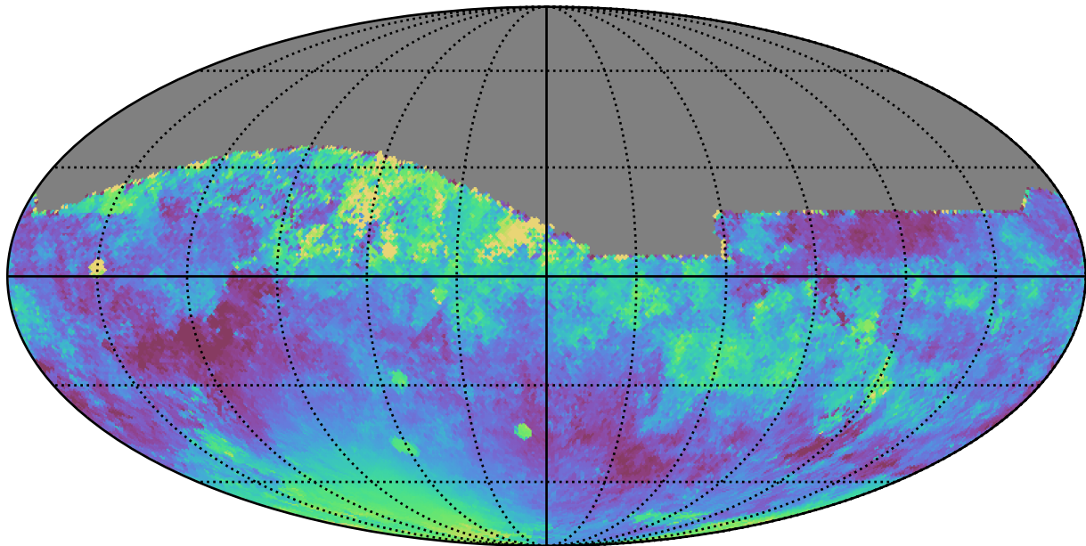
too_ignore_100_4v3.4_10yrs All sky z band: Median moonDistance
