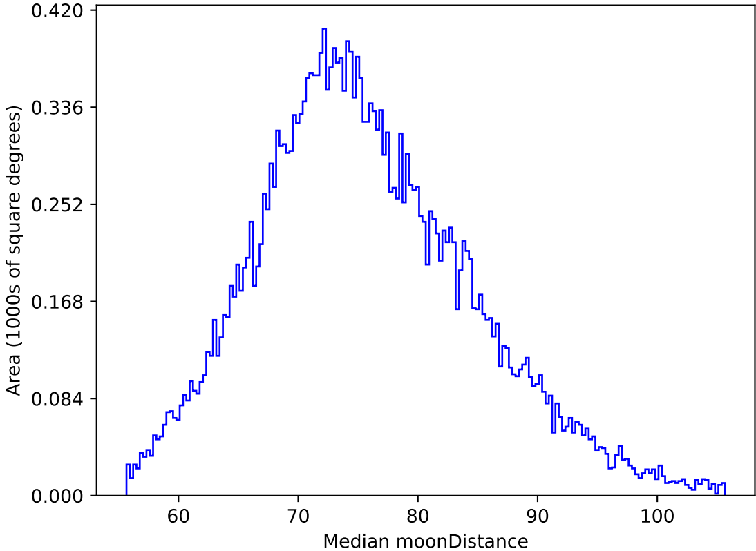
too_ignore_100_4v3.4_10yrs All sky z band: Median moonDistance
