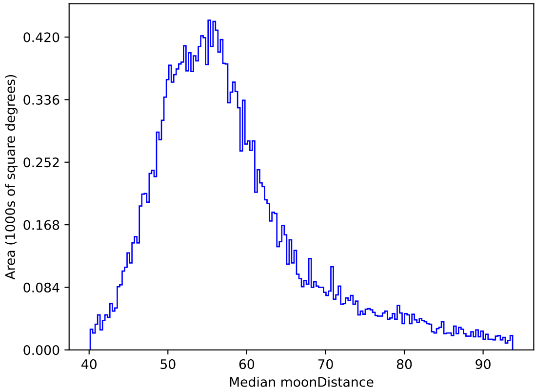
too_ignore_100_4v3.4_10yrs All sky y band: Median moonDistance
