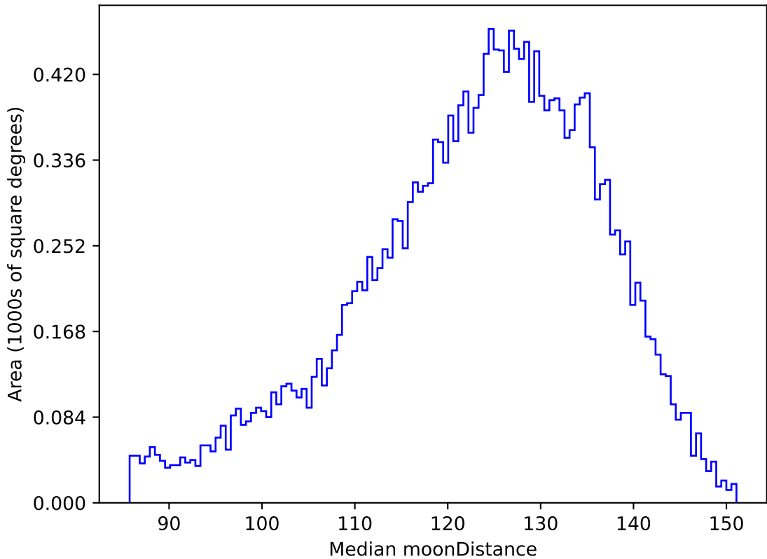
too_ignore_100_4v3.4_10yrs All sky u band: Median moonDistance
