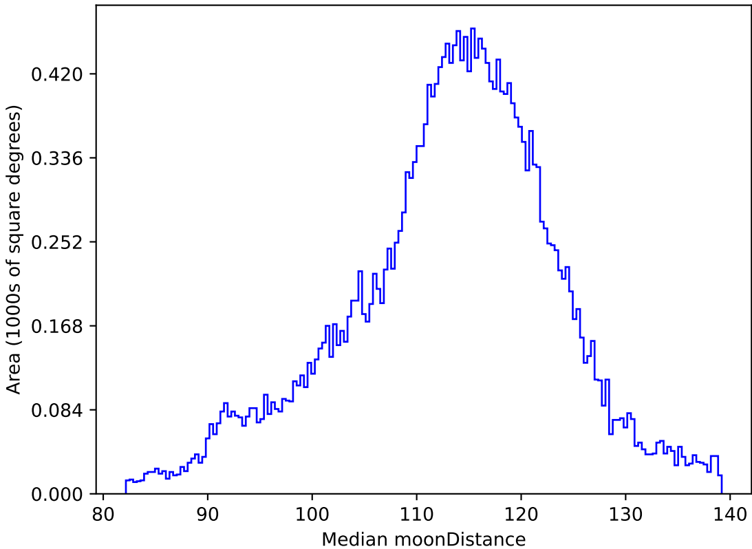
too_ignore_100_4v3.4_10yrs All sky r band: Median moonDistance
