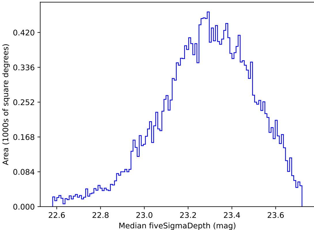
too_ignore_100_4v3.4_10yrs Yr 1 u band: Median fiveSigmaDepth
