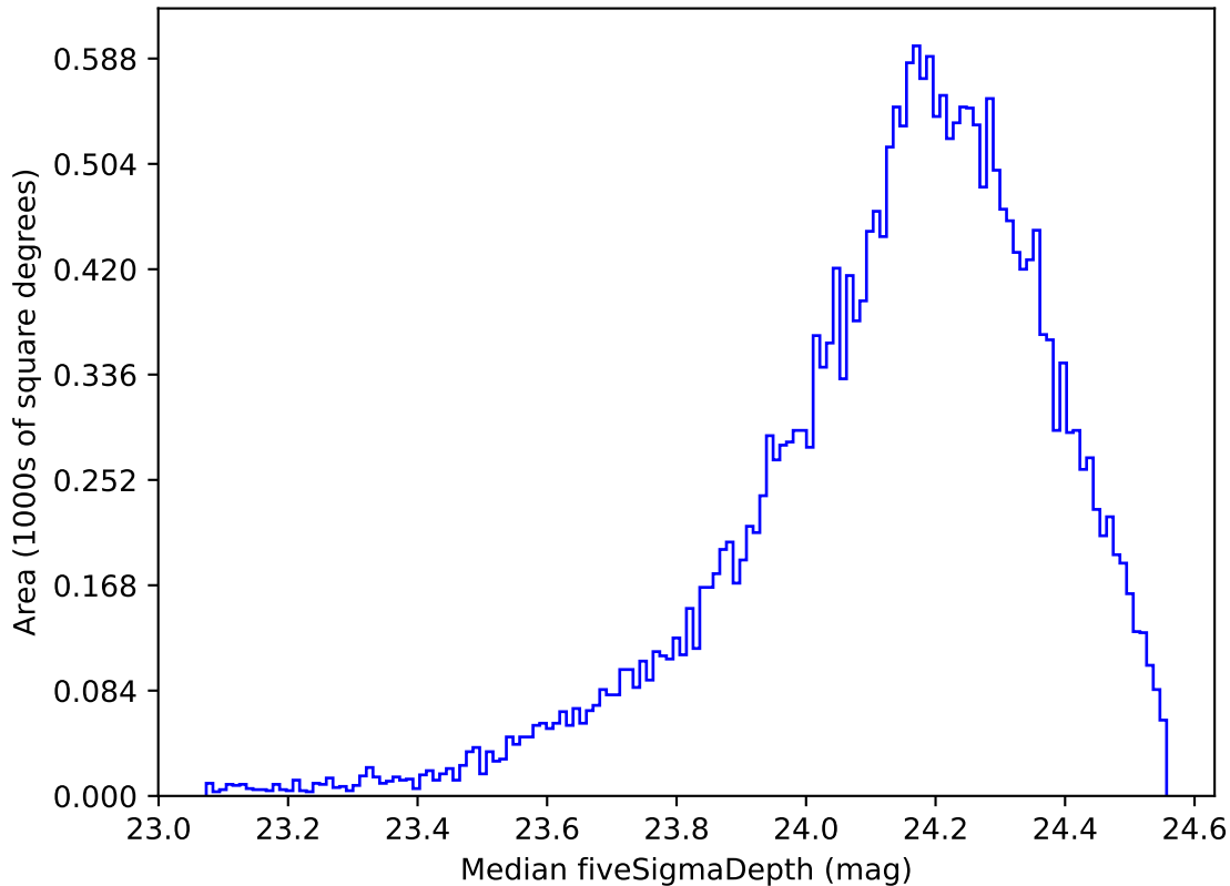
too_ignore_100_4v3.4_10yrs Yr 1 r band: Median fiveSigmaDepth
