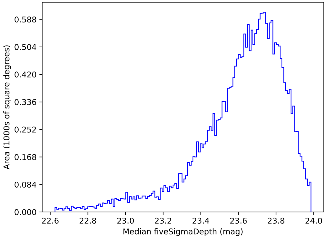
too_ignore_100_4v3.4_10yrs Yr 1 i band: Median fiveSigmaDepth
