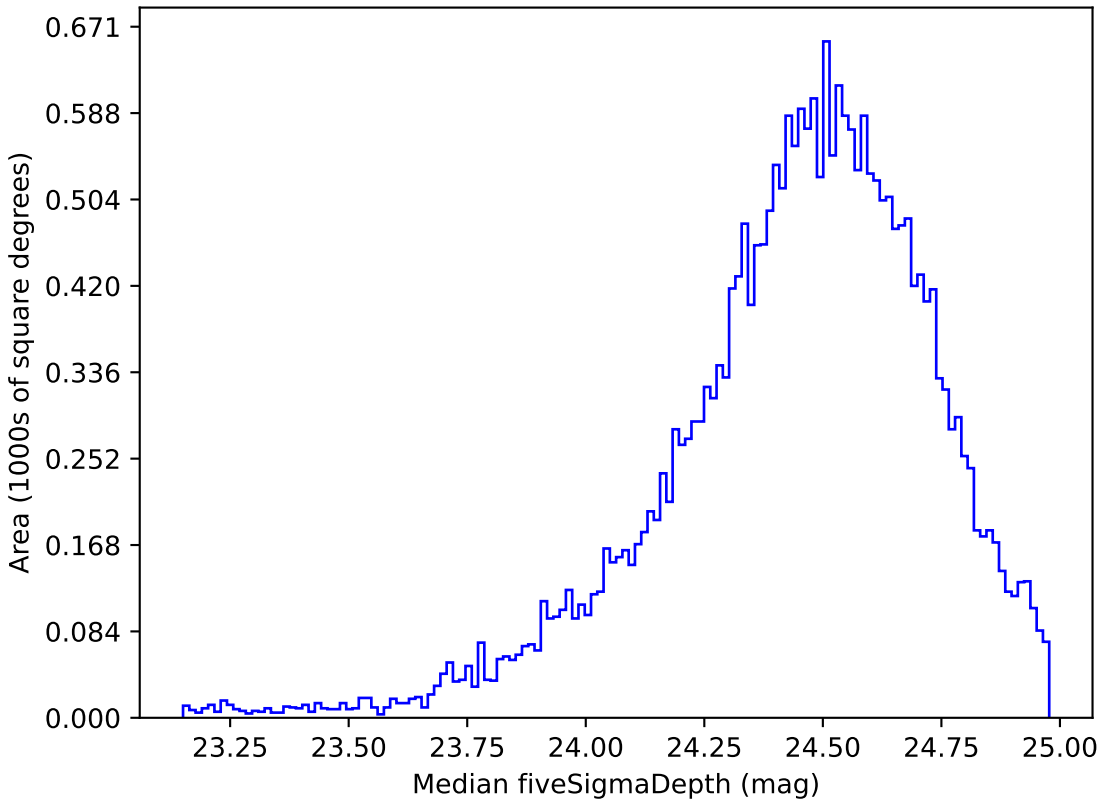
too_ignore_100_4v3.4_10yrs Yr 1 g band: Median fiveSigmaDepth
