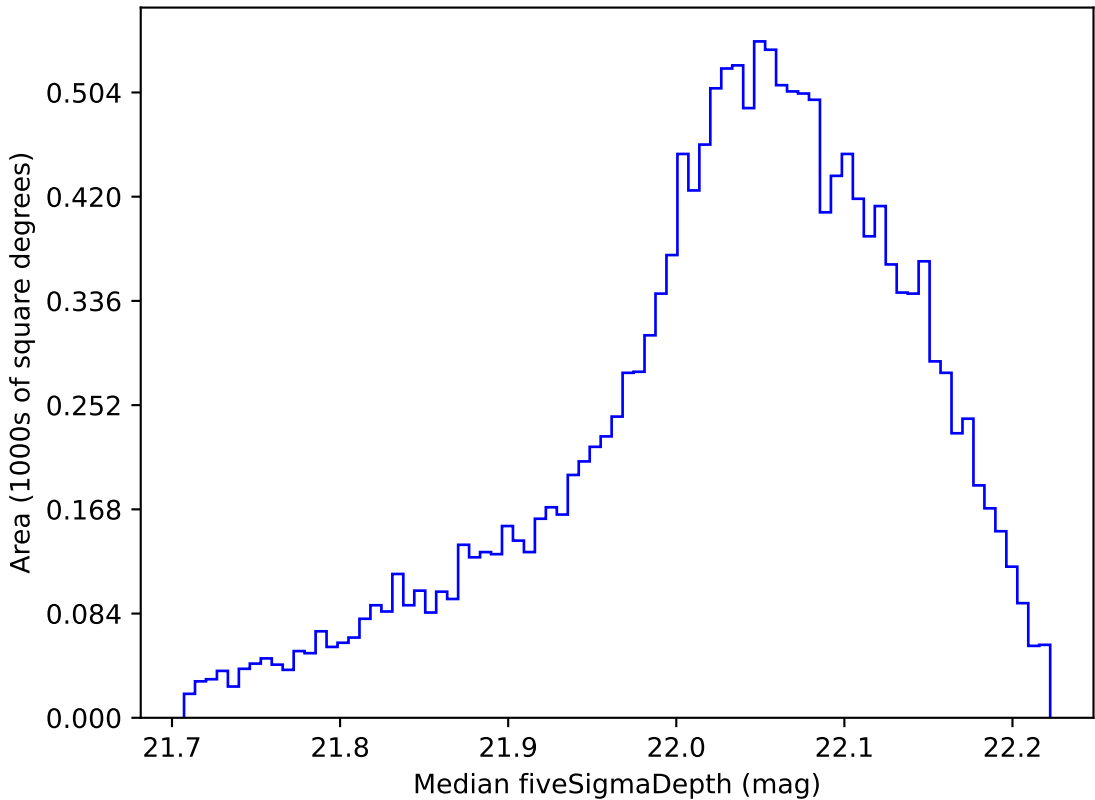
too_ignore_100_4v3.4_10yrs WFD y band: Median fiveSigmaDepth
