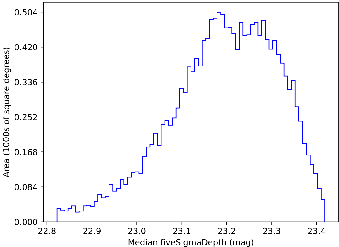
too_ignore_100_4v3.4_10yrs WFD u band: Median fiveSigmaDepth
