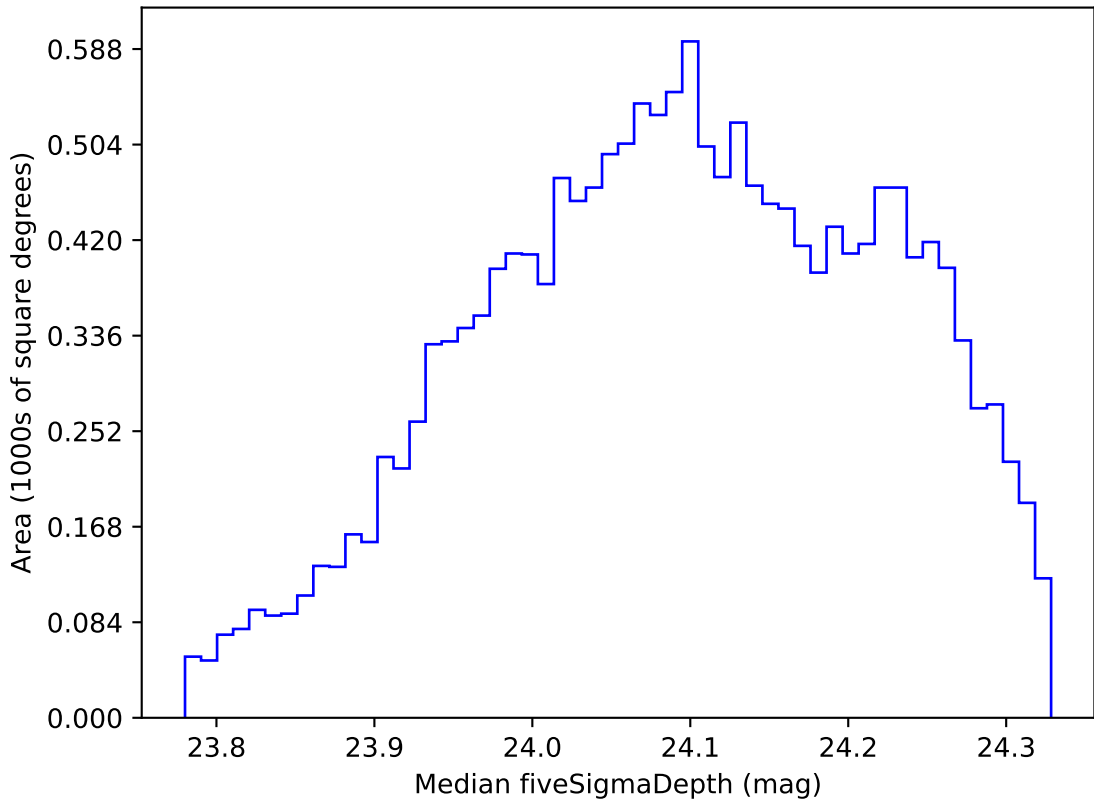
too_ignore_100_4v3.4_10yrs WFD r band: Median fiveSigmaDepth
