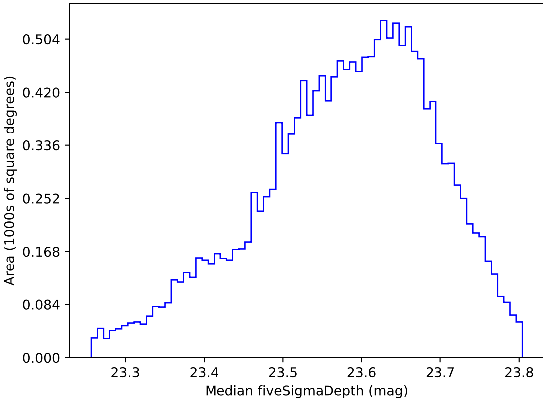
too_ignore_100_4v3.4_10yrs WFD i band: Median fiveSigmaDepth
