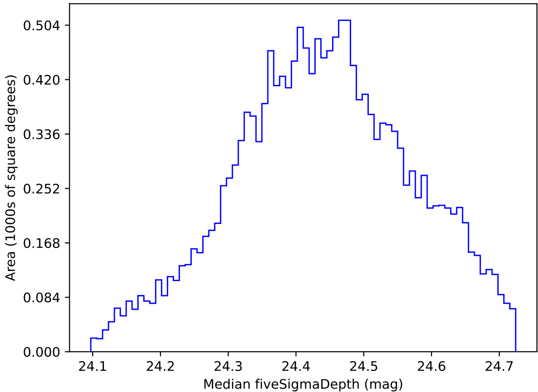
too_ignore_100_4v3.4_10yrs WFD g band: Median fiveSigmaDepth
