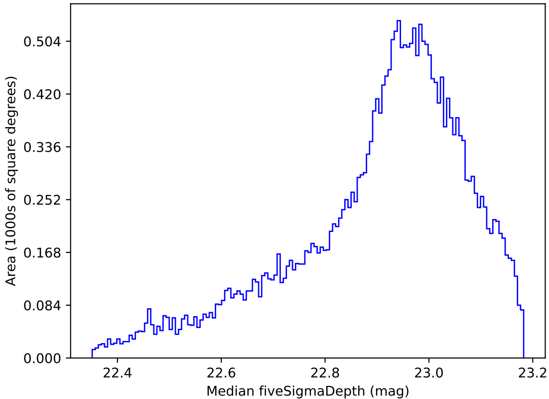
too_ignore_100_4v3.4_10yrs All sky z band: Median fiveSigmaDepth
